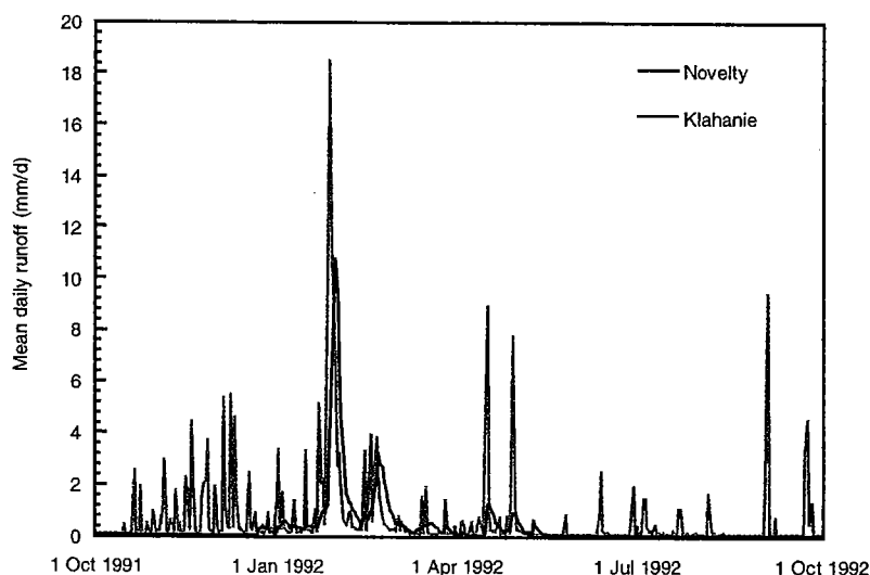
FIGURE 2. Runoff during water year 1992 for two headwater catchments in western Washington. At the time of data collection, Novelty was a fully forested 37-ha catchment; Klahanie was a fully built-out 17-ha residential catchment.
