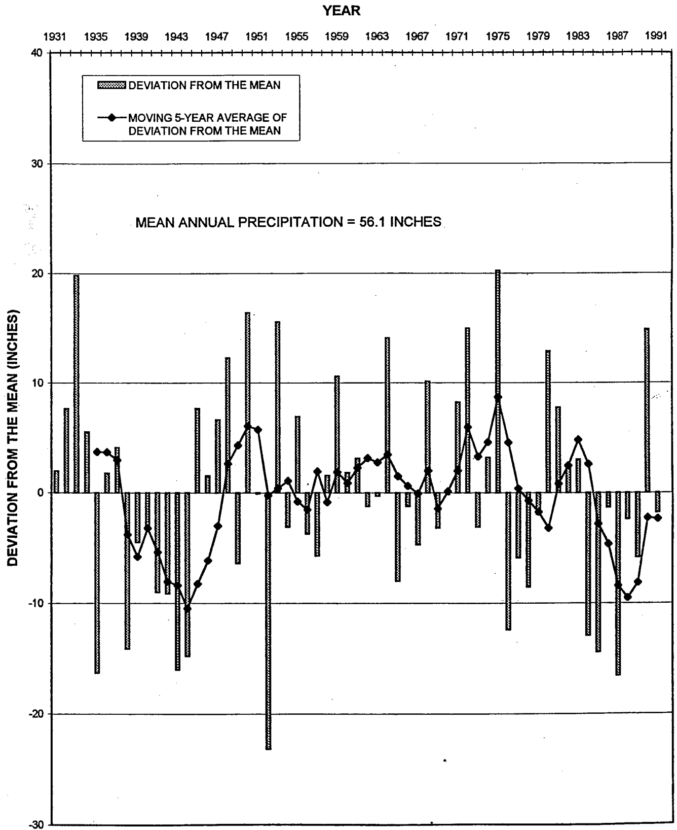
FIGURE 4c - 1931-1991 PRECIPITATION AT LANDSBURG
